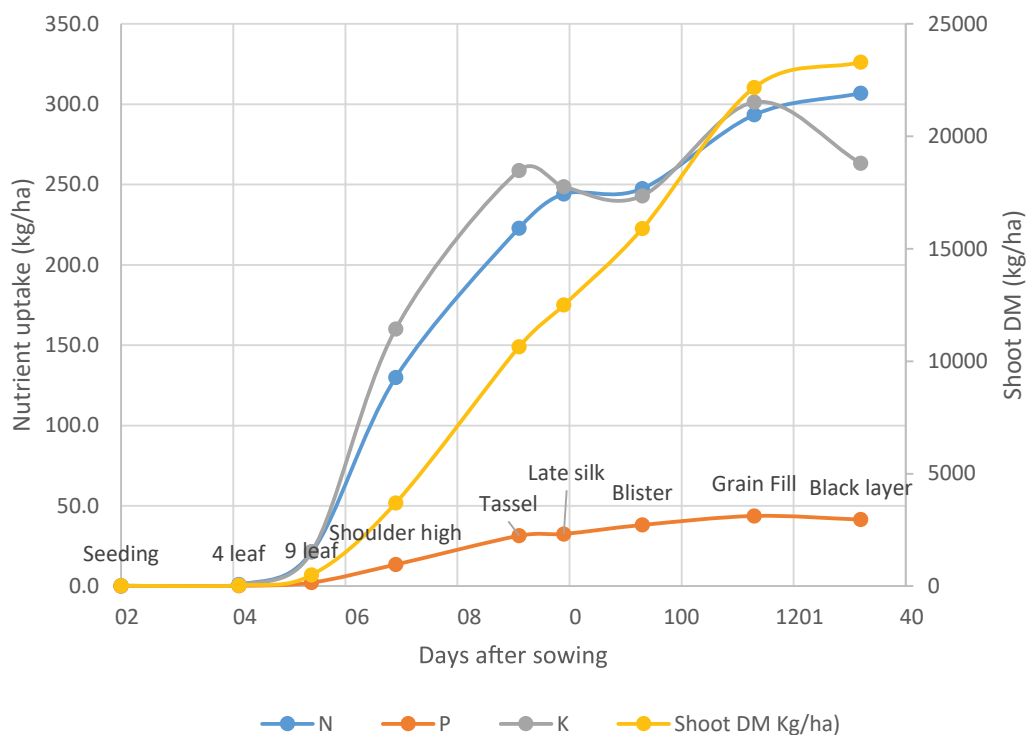
Figure 1: Nitrogen, phosphorus and potassium uptake patterns for an 11t/ha grain corn crop (Purdue University 1995)
